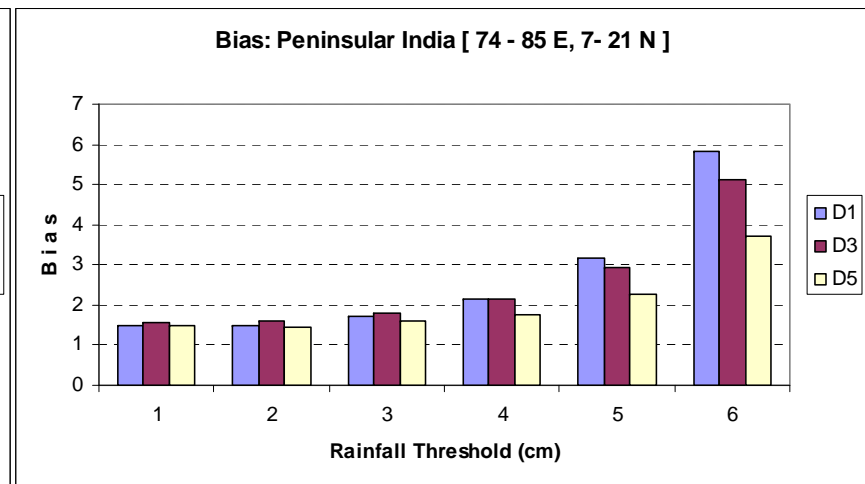
Fig. 4: Rainfall threshold based skill scores for Peninsular India Region for the 2009 monsoon season
